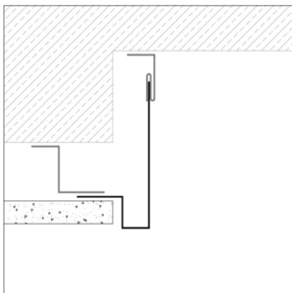
Window reveal
