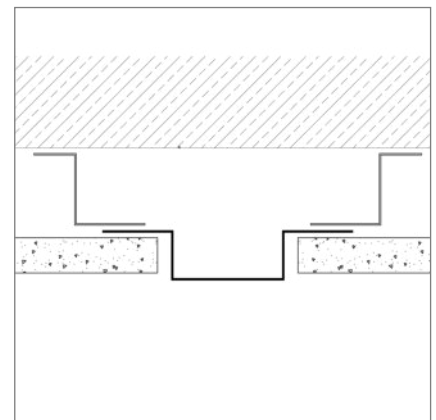
Pilaster strip
